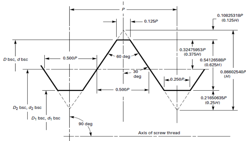
Fig. 1 Basic Profile for UN and UNR Screw Threads
